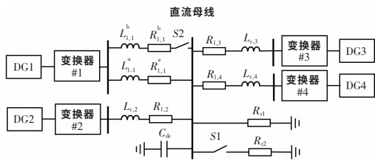
图 9 直流微网结构示意图 Fig.9 Structure diagram of the studied DC microgrid
