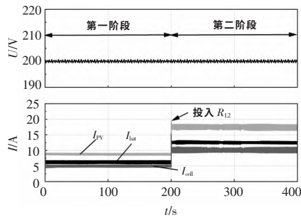
图 8 负荷突变时的仿真结果 Fig.8 Simulation results during load mutation
