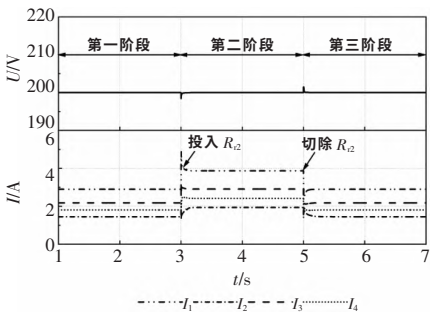
图 10 负荷突变时的仿真结果 Fig.10 Simulation results during load fluctuation
