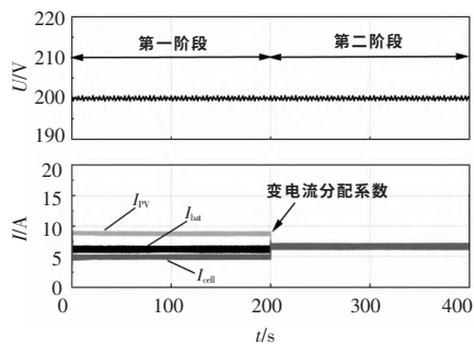
图 7 电流分配系数改变时的仿真结果 Fig.7 Simulation results when the current distribution coefficients change
