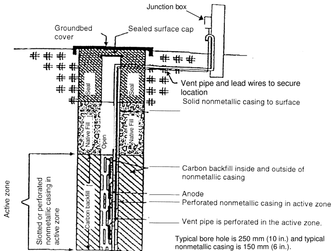
Figure A5: Typical Replaceable Closed Hole
