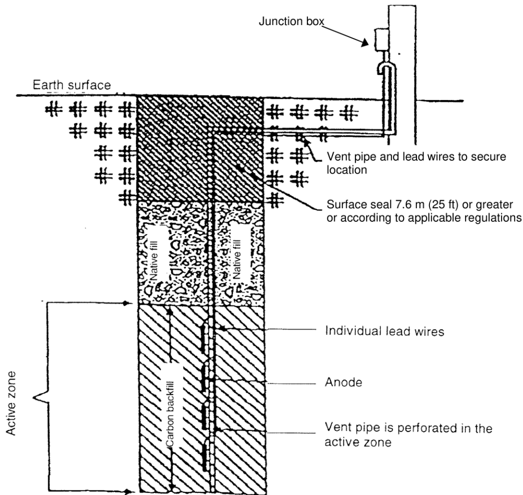
Figure A1: Closed Hole
