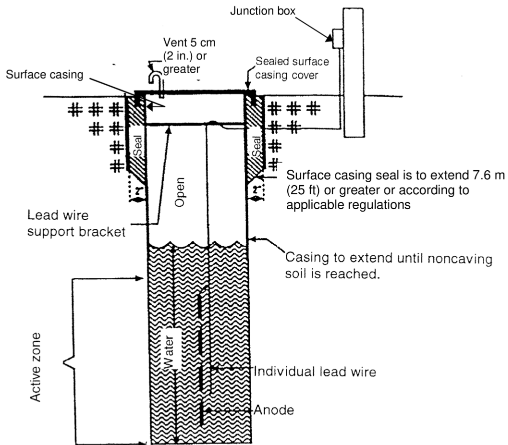
Figure A3: Open Hole with Surface Casing
