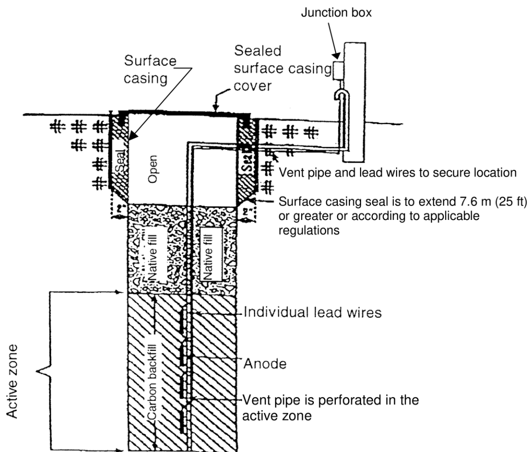
Figure A2: Closed Hole with Surface Casing
