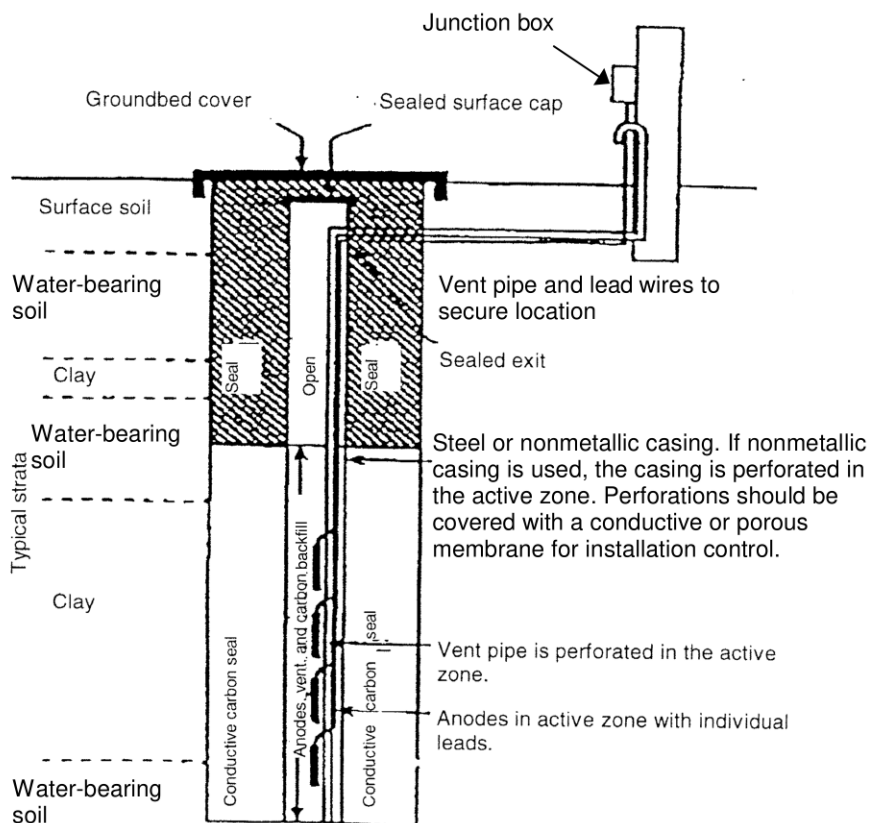
Figure A4: Environmentally Addressed System
