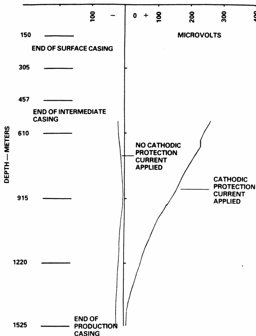
FIGURE A.2—Typical Casing Potential Profile Plot
