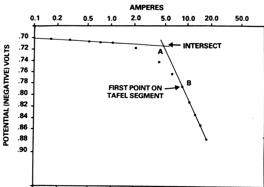
FIGURE B.2—Sample E-Log-I Plot
