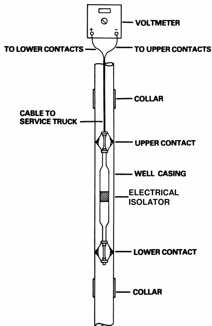
FIGURE A.1—Casing Potential Profile Tool
