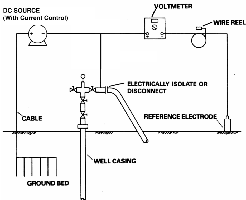
FIGURE B.1—Equipment Set-Up for E-Log-I Test
