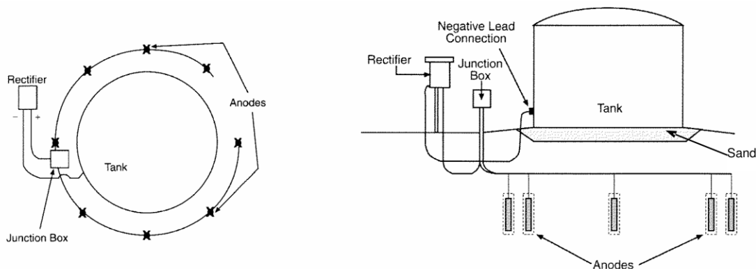
Figure 4: Vertically Drilled Anode CP System
