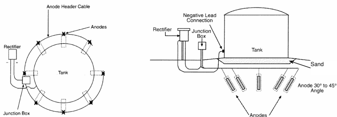
Figure 5: Angled Anode Cathodic Protection System
