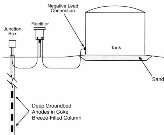
Figure 6: Deep Anode Groundbed
