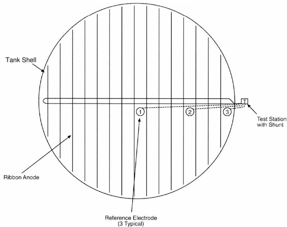
Figure 9: Typical Double-Bottom Galvanic Anode Design
