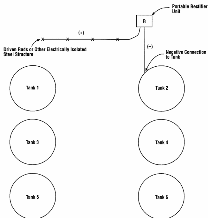
Figure 2: Temporary Groundbed for Current Requirement Testing
